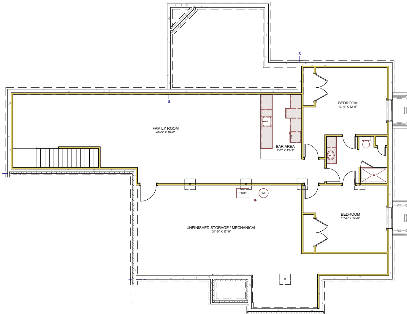
FINISHED BASEMENT LAYOUT PROPOSED FINISHED SQFT = 1,405 sqft
